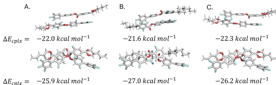
Fig. 8 Minimum energy configurations of DIO in the slipped antiparallel (top) and twisted antiparallel (bottom) configurations (A); CIO in slipped antiparallel (top) and twisted antiparallel (bottom) configurations (B); DIO(-F) in the slipped antiparallel (top) and twisted antiparallel (bottom) (C). \Delta E_{\text{cplx}} is the counterpoise complexation energy at the DFT B97D3/cc-pVTZ level.
