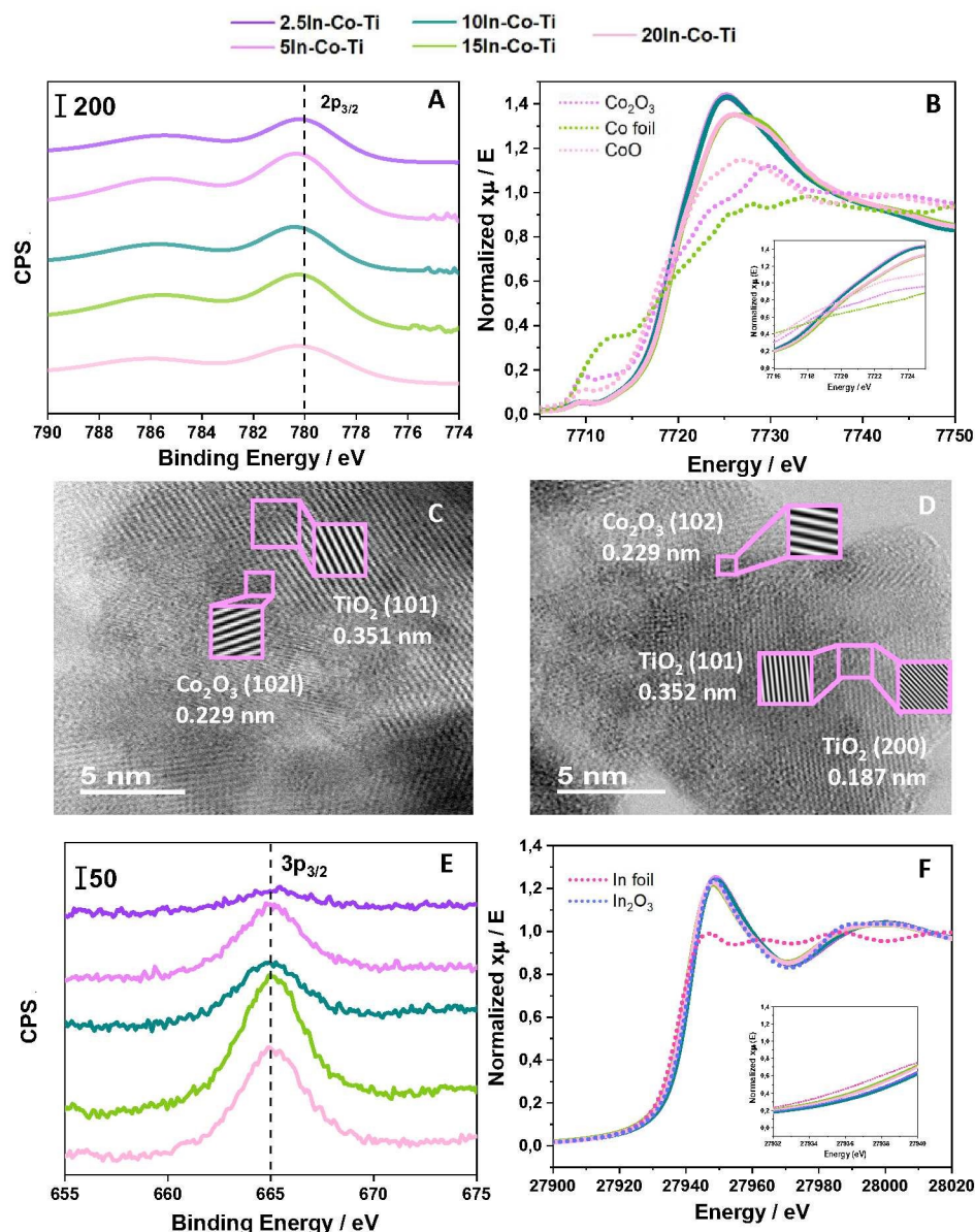
Figure 3. (A) Co 2p_{3/2} XPS spectra for the xIn-Co-Ti samples. (B) Co K-edge XANES spectra for the xIn-Co-Ti catalysts and reference samples. (C) TEM micrographs for the 2.5In-Co-Ti sample. (D) TEM Micrographs for the 10In-Co-Ti sample. (E) In 3p_{3/2} XPS spectra for the xIn-Co-Ti samples. (F) In K-edge XANES spectra for the xIn-Co-Ti catalysts and reference samples.
