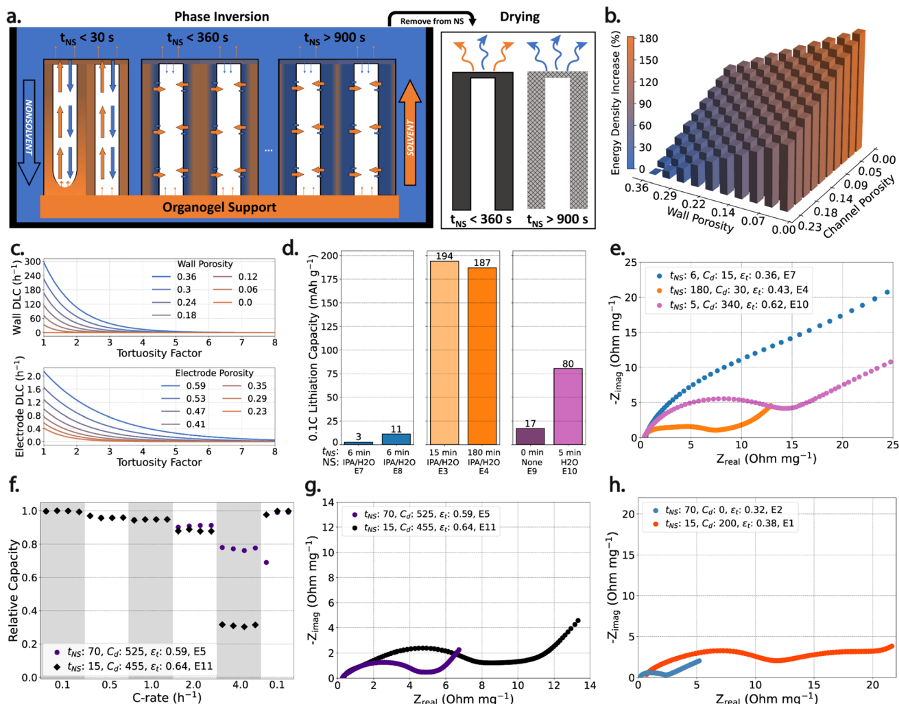
Fig. 3 (a) Schematic illustration of channel-like pore formation through the opposing diffusion of solvent and nonsolvent in phase inversion. When quenched after a short immersion time ( t_{\text{NS}} < 360 s), the result is a higher fraction of solvent (orange) remaining in the material-dense wall, leading to substantial densification during drying and lower accessibility to the active material. Alternatively, diffusion can be allowed to proceed for longer times ( t_{\text{NS}} > 900 s), which results in highly porous walls after drying and carbonization. (b) Three-dimensional bar plot demonstrating how energy density increases when independently replacing wall and channel porosity with active material. These calculations are based on the best performing electrode E5 at 4 C as the baseline, which has a \epsilon_t = 0.59 that was divided into a wall porosity of 0.36 and a channel porosity of 0.23 (left corner). (c) The diffusion limited C-rate (DLC) of a single wall (top) and the full electrode (bottom) is plotted against values of tortuosity factor for various wall and electrode total porosities. (d) Bar plot of the experimental 0.1 C lithiation capacity achieved by electrodes with various nonsolvent types, immersion times ( t_{\text{NS}} in minutes) and channel density ( C_d in channels per \text{mm}^2 ). (e) Electrochemical impedance spectroscopy (EIS) presented as a Nyquist plot showing electrodes whose 0.1 C capacity is plotted in the first (E7), fourth (E4) and sixth (E10) column in (d) showing the trend of decreasing resistance with longer t_{\text{NS}} and replacement of isopropanol (IPA) with water in the nonsolvent bath. The full and areal Nyquist plots are shown in SI Fig. S2. (f) The relative capacity at varied C rates of two electrodes with similar architecture and different nonsolvent immersion time ( t_{\text{NS}} in minutes), illustrating the impact that vitrification-induced tortuosity in the secondary porosity has on high-C-rate performance. (g) EIS Nyquist plots of the two electrodes in (f) demonstrating the differing resistance between electrodes with similar C_d and \epsilon_t but different t_{\text{NS}} of 70 and 15 minutes. (h) EIS Nyquist plots of two low-porosity electrodes with C_d of 0 and 200 \text{mm}^{-2} , respectively, demonstrating the sensitivity of EIS to the local microstructure around the LTO particles but not C_d nor showing a correlation to high-rate lithiation capacity (compare to Fig. 2a). Area normalized EIS Nyquist plots for (g and h) can be found in Fig. S3. The legends in plots (d–h) reference the electrode identifier from Tables S1 and S2.
