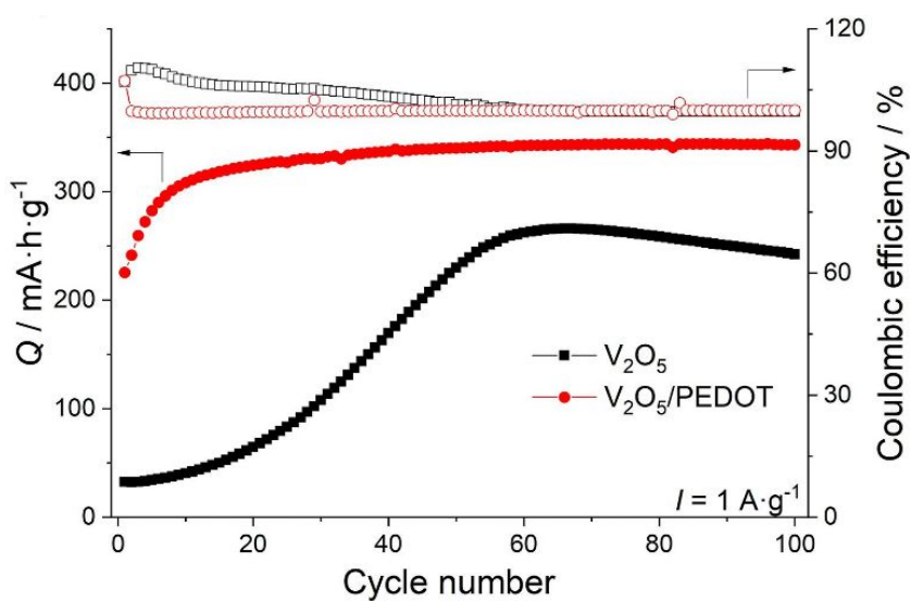
Figure 7. Electrochemical performance of V_2O_5 and V_2O_5 /PEDOT electrodes: cycle performance at 1 \text{ A}\cdot\text{g}^{-1} . Reprinted from Ref. [66], copyright (2022), with permission from Elsevier.
