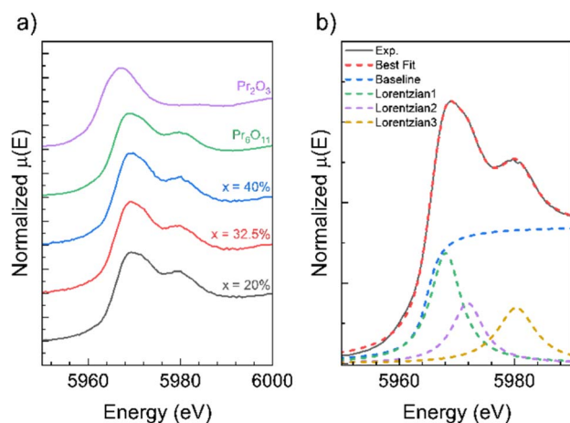
Fig. 6 (a) Pr L 3 absorption of Pr in Ce x (SmPrLaY) 1-x O 2-δ and measured standards and (b) an example of fitting procedure performed on Pr 6 O 11 .
