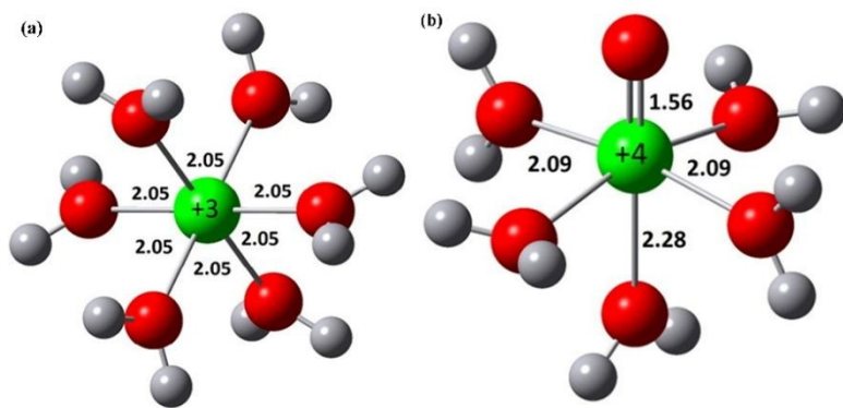
10 Fig. 3 Structures of (a) V^{3+} and (b) V^{4+} ions and their first solvation shell water 11 molecules by DFT 44 (Reprinted with permission of Elsevier) 12
