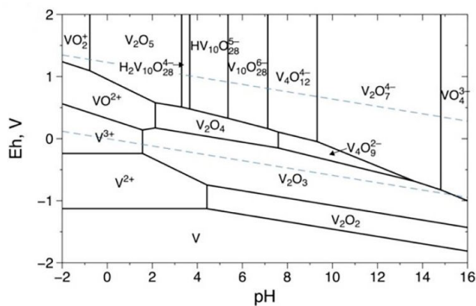
7 Fig. 2. Eh–pH diagram for vanadium species at [V]=1M 43 (Reprinted with permission 8 of American Chemical Society) 9
