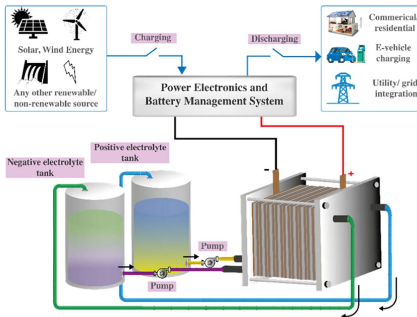
Fig. 1 VFB energy storage schematic 45 (reprinted with permission from Springer Nature).
