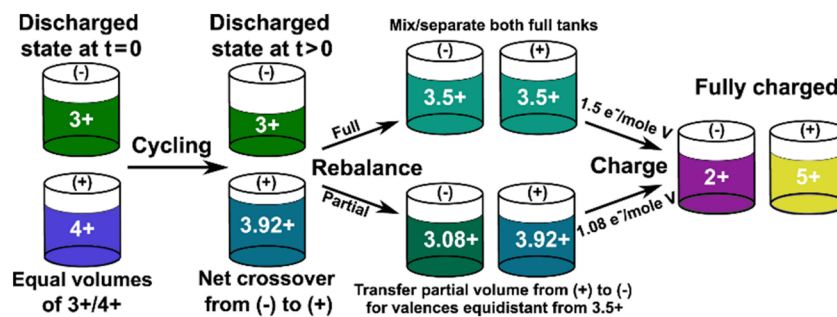
Fig. 21 Schematic of the full and partial rebalancing techniques 26 (reprinted with permission from Elsevier).
