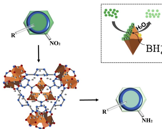
Fig. 5 Schematic illustration of the proposed mechanisms of the conversion of NP to AP by MIL-101(Fe)/ SiO_2 . Reprinted with permission from ref. 88. Copyright 2020, Elsevier.
