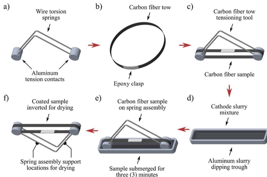
Fig. 6 Illustration of various stages in the coating process of a CF cathode: (a) assembling of a fiber torsion tool with wire a torsion spring and aluminium tension contact, (b) fiber tow of the sample cut and clasped by epoxy, (c) fiber sample positioned over spring tensioner after curing the epoxy, (d) slurry mixture of the cathode mixed poured into aluminium through dipping, (e) sample of fiber tow submerged into cathode slurry and (f) spring tensioner fiber tow inverted to drying. Reproduced with permission from ref. 32. Copyright (2022), American Chemical Society.
