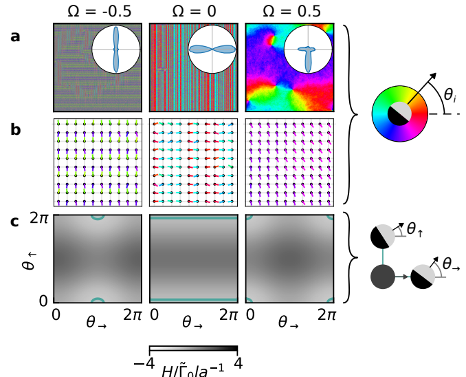
FIG. 5 | Ordering on a square lattice. a , b , Snapshots of 500 \times 500 spins ( a ) and close-up views of 10 \times 10 spins ( b ) for turn-towards interactions with \tilde{\Gamma}_0 l/a = 50 and different distance-dependence parameters \Omega = -0.5, 0, 0.5 . Color represents particle orientation. The insets in a show the angular distribution. c , Effective energy H between a particle oriented along the x axis and two neighbors: one along the x axis with orientation \theta_{\rightarrow} , and one along the y axis with orientation \theta_{\uparrow} (see schematic). The turquoise contours enclose regions with 90% of the probability p(\theta_{\rightarrow}, \theta_{\uparrow}) \propto e^{-H} .
