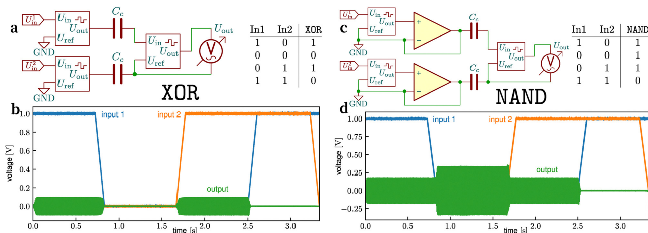
Fig. 5 Circuit diagrams of a XOR-pre-gate (a) and a NAND-pre-gate (c) constructed by combining three Memriks oscillators from Fig. 2 (represented here by the three boxes), either coupled solely via capacitors (a) or with the addition of two operational amplifiers (c). Time traces of the two input voltages (blue and orange) representing the four consecutive binary states 10, 00, 01, 11. The resulting quasi-binary output voltage (green), which is either quiescent or oscillating, is shown in (b) for circuit (a), revealing XOR behavior, and in (d) for circuit (c), exhibiting NAND behavior. The corresponding truth tables are shown next to the circuit diagrams.
