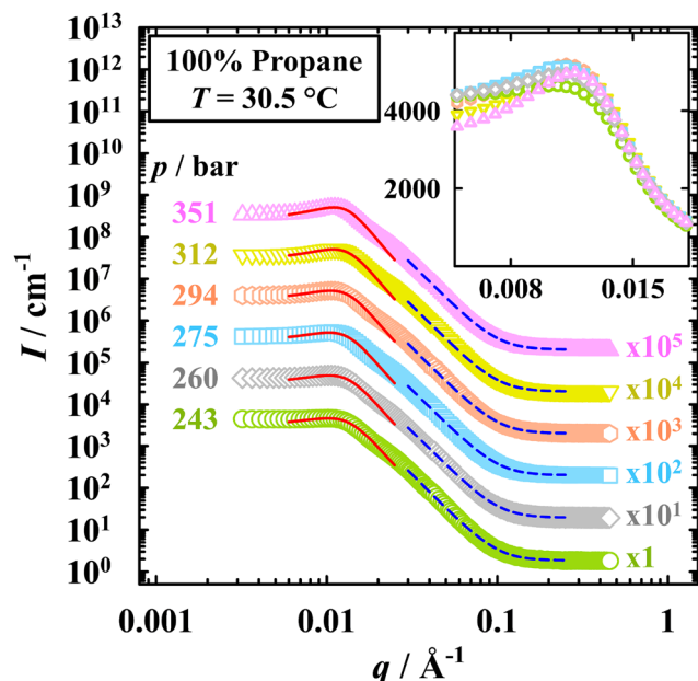
Fig. 5 Pressure-dependent bulk contrast SANS curves for the micro-emulsion system containing 100 wt% propane, recorded isothermally at T = 30.5\text{ °C} and \phi_C = 0.064 . Curves are displaced by a factor of 10 (243 bar unscaled). Peak region analyzed via the Teubner–Strey model 32 (red solid lines); high q analyzed with Porod's law, taking into account the diffuseness of the amphiphilic film 33,34 (blue dashed lines). The measurement at 200 bar, measured outside of the one-phase region, no longer exhibits the typical features of bicontinuous microemulsions (cf. Fig. S5 and S6, ESI†). Inset: Unscaled close-up of the peak region with linear I axis. Fits are omitted for better visibility.
