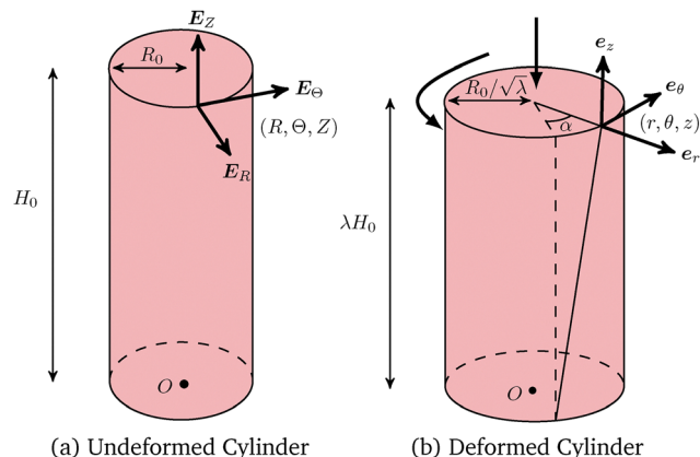
Fig. 6 (a) Undeformed and (b) deformed cylinder. Torque and normal force must be applied at the end of the cylinder to maintain the torsion deformation.
