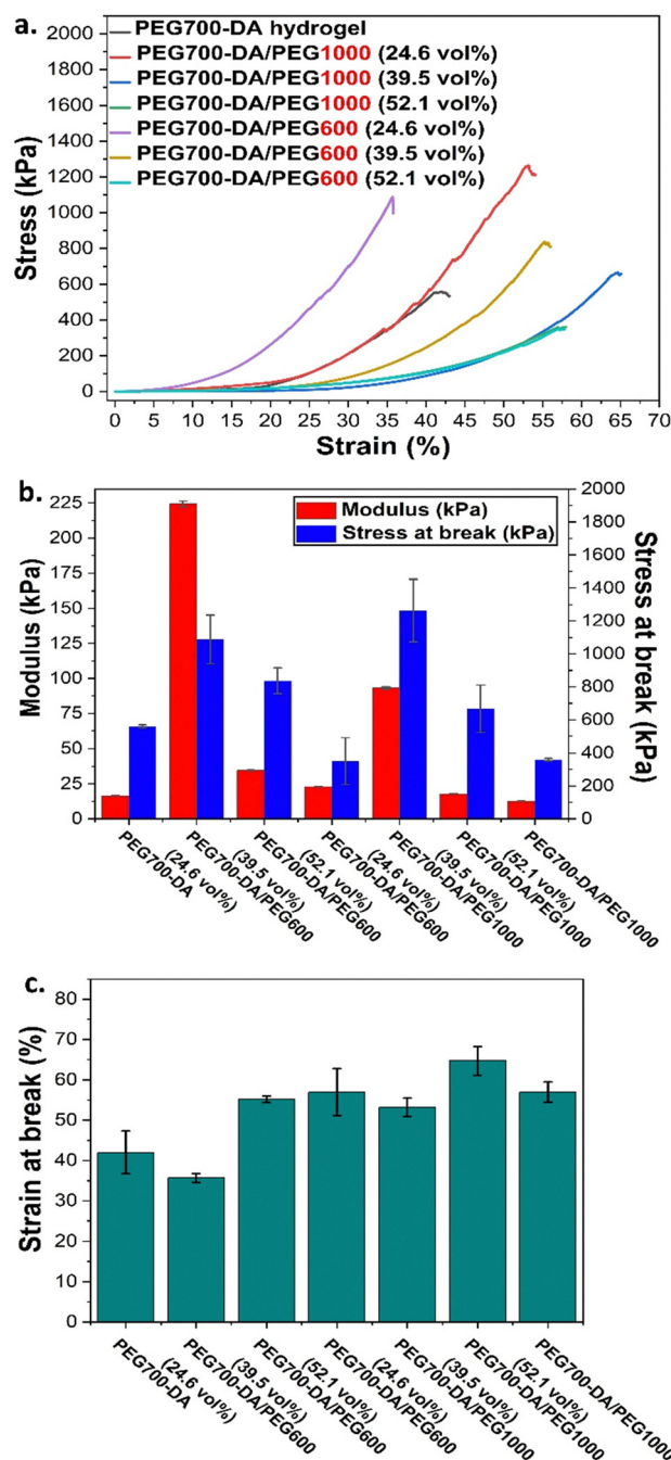
Fig. 2 (a) Representative compression curves for pristine PEG700-DA/PEGx hydrogels (b) modulus and stress at break data and (c) strain at break results. Data given as mean \pm SD of the average of at least n = 8 samples.
