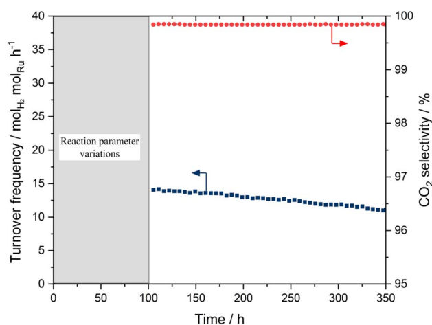
Fig. 3 Long-term activity (blue square, TOF) and CO 2 selectivity (red circle) in continuous methanol steam reforming on BiCat SLP catalyst. Reaction conditions: p = 0.1 MPa; n(\text{MeOH}:\text{H}_2\text{O}) = 1 ; T = 423 K; m_{\text{cat}} = 1050 g; \text{GHSV} = 40 h -1 . Catalyst composition: \Phi_{\text{Ru}} = 50 \mu\text{mol}_{\text{Ru}} \text{ g}_{\text{support}}^{-1} ; \Pi_{\text{Ru-1-Ru-2}} = 5.6 ; \omega_{\text{CsOH,syn}} = 20 wt%; alumina support material 1.8 mm \varnothing .
