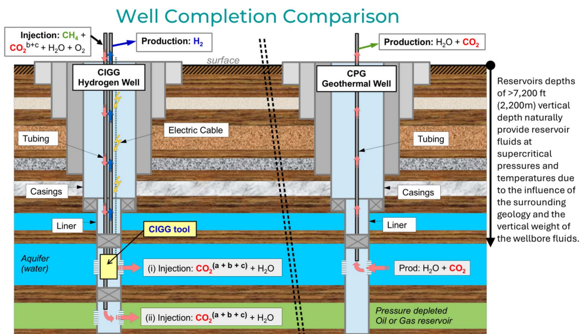
Fig. 5 An illustration of an enhanced geothermal well completion utilizing CIGG. CO 2 a = CO 2 produced from CH 4 reformation, CO 2 b = externally sourced CO 2 from industry, CO 2 c = biogas natural CO 2 content, CIGG = Carbon Injection and Gasification Geothermal. CPG = CO 2 plume geothermal.
