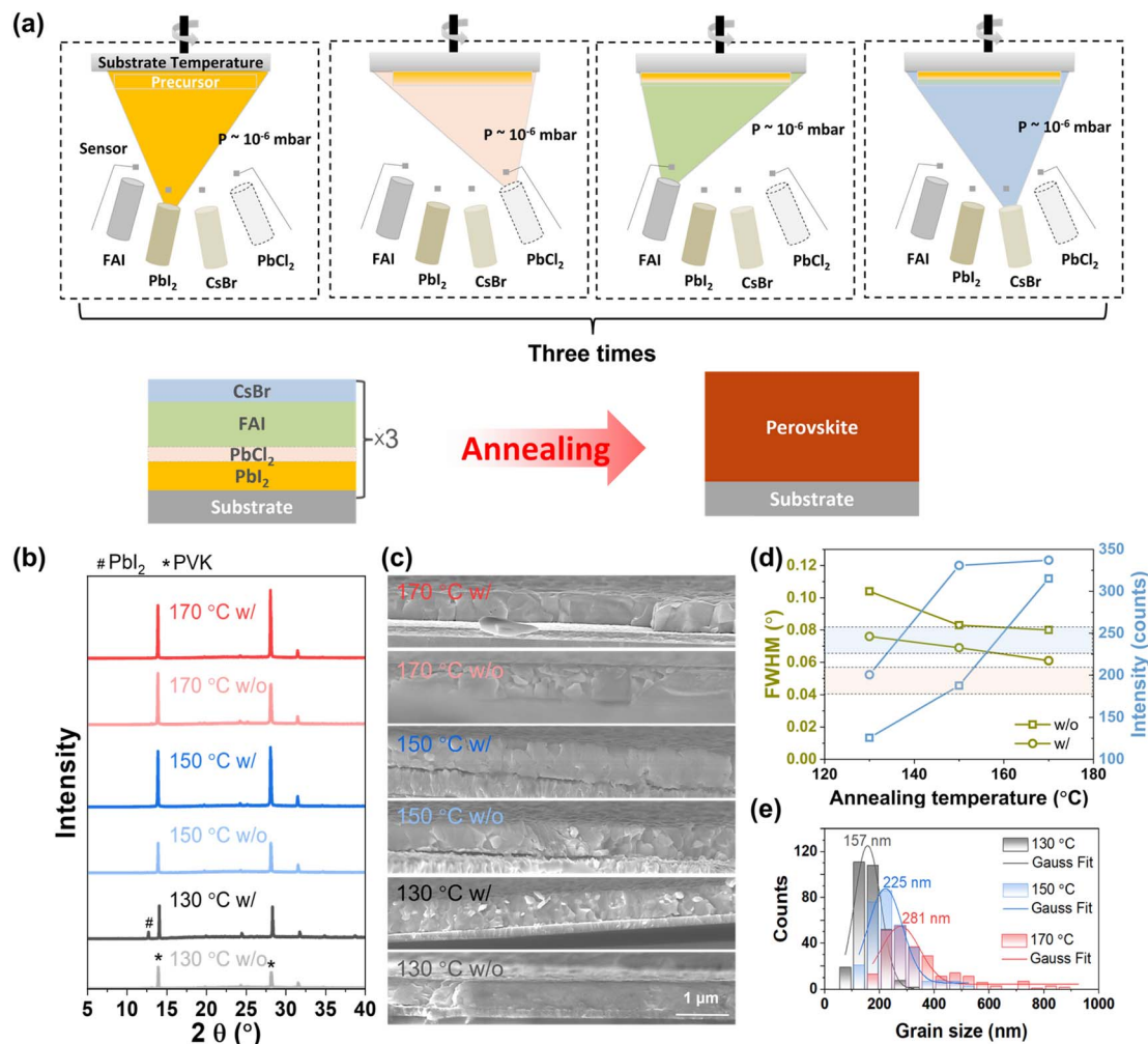
Fig. 1 (a) Schematic illustration of sequential thermal evaporation to prepare a PVK absorber. (b) XRD patterns of PVK films w/o and w/ \text{PbCl}_2 subjected to different annealing temperatures for 10 minutes, and the XRD patterns are shifted for an easier comparison. Both the diffraction peak of \text{PbI}_2 and PVK are illustrated with different symbols. (c) Cross-sectional SEM of PVKs at varying annealing temperatures (10 minutes) for both w/o and w/ \text{PbCl}_2 samples. (d) FWHM and absolute peak intensities of the (100) crystal plane of w/o and w/ \text{PbCl}_2 samples as a function of annealing temperature. (e) Grain size distribution of PVK films w/ \text{PbCl}_2 at different annealing temperatures. Grain sizes were measured using ImageJ software and data were extracted from top view SEM images in Fig. S1†
