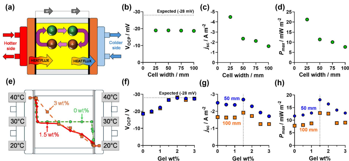
Fig. 2 The top row shows (a) a cartoon of the water–water heat exchanged thermogalvanic cell; and the measured (b) open-circuit voltage ( V_{\text{OCp}} ), (c) short-circuit current density ( j_{\text{sc}} ) and (d) the maximum power density ( P_{\text{max}} ) measured for \text{K}_3/\text{K}_4[\text{Fe}(\text{CN})_6] as a function of cell width when exposed to \Delta T = 20 \text{ K} ( T_{\text{cold}} = 20^\circ \text{C} , T_{\text{hot}} = 40^\circ \text{C} ). The bottom row summarises the results from varying the wt/v% of polyacrylate gel added to \text{K}_3/\text{K}_4[\text{Fe}(\text{CN})_6] , showing (e) the temperature gradient measured across the 100 mm cell for 0, 1.5, and 3 wt% (data tabulated in the ESI†), and the measured (f) V_{\text{OCp}} , (g) j_{\text{sc}} and (h) P_{\text{max}} for 50 mm (blue circles) and 100 mm (orange squares) wide thermocells.
