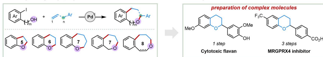
Scheme 1 Pd-catalyzed migratory cycloannulation reaction.
