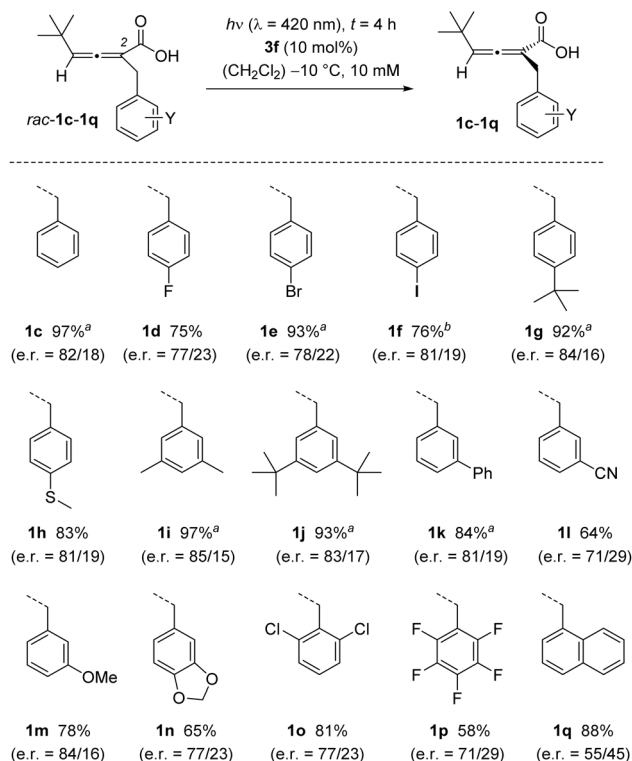
Scheme 3 Photochemical deracemization of 2,3-allenoic acids rac - 1c to rac - 1q as catalysed by chiral Brønsted acid 3f (50 \mu\text{mol} scale).
