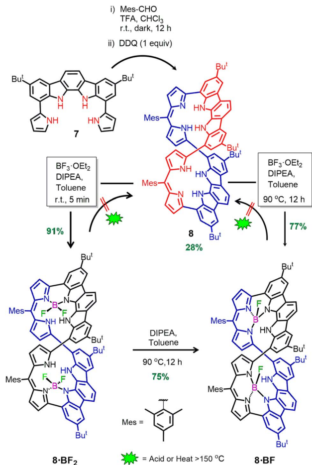
Scheme 1 Synthesis of macrocycle 8 , bis- \text{BF}_2 complex 8 · \text{BF}_2 , and bis-BF complex 8 · BF . Bu t = tert -butyl, TFA = trifluoroacetic acid, DDQ = 2,3-dichloro-5,6-dicyano-1,4-benzoquinone, DIPEA = diisopropylethylamine.
