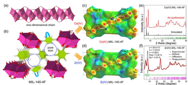
Fig. 2 (a) One-dimensional inorganic subunit of the metal oxide chain in MIL-140-4F. (b) Illustration of the crystal structure and pore chemistry of MIL-140-4F. (c and d) The Hirshfeld surface with d_e (electrostatic potential) and binding sites in Ce IV - (c) and Zr IV -MIL-140-4F (d) (red-to-blue color indicates the high-to-low transition of electron density). (e) Experimental and simulated PXRD patterns of Ce IV -MIL-140-4F. (f) Experimental (black) and Pawley refined (red) PXRD patterns of Zr IV -MIL-140-4F. Reproduced from ref. 29 with permission from Wiley-VCH, copyright 2021.
