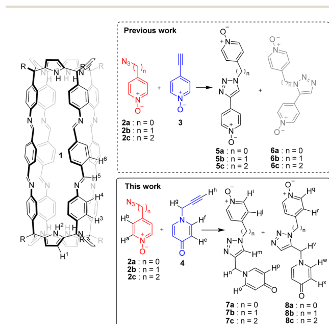
Fig. 1 Molecular structure of octa-imine cage 1 and scheme of the 1,3-dipolar cycloaddition reaction between azido- (2a–2c) and ethynyl (3 or 4) producing the two regioisomeric 1,4- (5 or 7) and 1,5- (6 or 8) disubstituted 1,2,3-triazoles. The corresponding proton assignments for octa-imine 1 , substrates 2 , and 4 , and products 7 and 8 are also shown.
