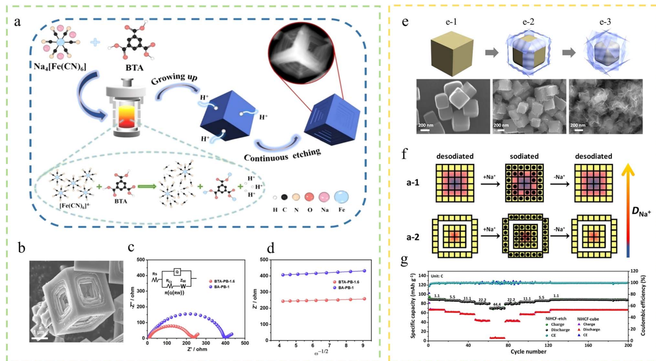
Fig. 12 (a) Scheme of the synthesis process of BTA-PB. (b) SEM images of BTA-PB-1.6. (c) EIS spectra of BTA-PB-1.6 and BA-PB-1. (d) Corresponding relationship between \text{Z}' and \omega^{-1/2} . 112 Copyright 2024, American Chemical Society. (e) Schematic diagrams accompanied by FESEM images of the NiHCF products after the etching time for (e-1) 0 hours, (e-2) 0.5 hours, (e-3) 6 hours. (f) Outside-in diffusion route of Na in NiHCF-cube and NiHCF-etch. (g) Rate performance of NiHCF-cube and NiHCF-etch. 113 Copyright 2017, American Chemical Society.
