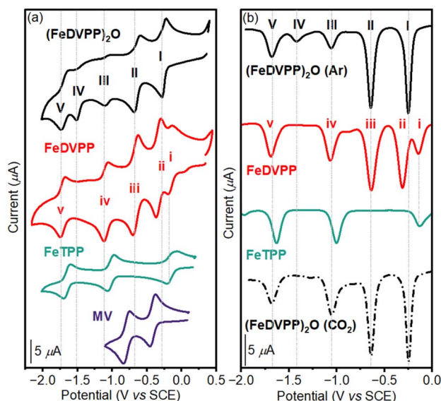
Fig. 1 (a) Cyclic voltammograms of 0.25 mM (FeDVPP) 2 O (black), 0.5 mM FeDVPP (red), 0.5 mM FeTPP (green), and 0.5 mM MV (purple) in DMF with 0.1 M [\text{Bu}_4\text{N}]\text{PF}_6 under Ar at 100 mV s −1 scan rate. (b) Differential pulse voltammograms of (FeDVPP) 2 O (black), FeDVPP (red) and FeTPP (green) in Ar, and (FeDVPP) 2 O in CO 2 (dash dot) [E step: 4 mV, amplitude: 50 mV, pulse width: 60 ms, sampling width: 20 ms, and pulse period: 500 ms].
