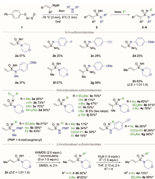
Scheme 1 Synthesis of N -H- and N -functionalised sulfonimidamides from BiPhONSO. Conditions for N -H sulfonimidamides: BiPhONSO (1.0 equiv.), alkenyl Grignard (1.0 equiv.), THF, -78\text{ }^\circ\text{C} , 3 min then amine (1.2–1.5 equiv.), -78\text{ }^\circ\text{C} to 0\text{ }^\circ\text{C} , 7 min. Functionalization of vinylsulfonimidamides: 1.0 equiv. of sulfonimidamide was used in all cases. a Et 3 N (1.5 equiv.), E + (1.1–1.5 equiv.), THF, 0\text{ }^\circ\text{C} to rt, 2–20 h; b pyridine (1.5–1.8 equiv.), E + (1.1–1.5 equiv.), THF, 0\text{ }^\circ\text{C} to rt, 3–16 h; c KHMDS (2.0 equiv.), E + (0–1.5 equiv.), DMSO, rt, 2 h; d p -tolyl boronic acid (2.3 equiv.), Cu(MeCN) 4 BF 4 (15 mol%), DMF, rt, O 2 , 24 h; e NaH (1.2 equiv.), MsCl (1.1 equiv.), THF, 0\text{ }^\circ\text{C} to rt, 18 h.
