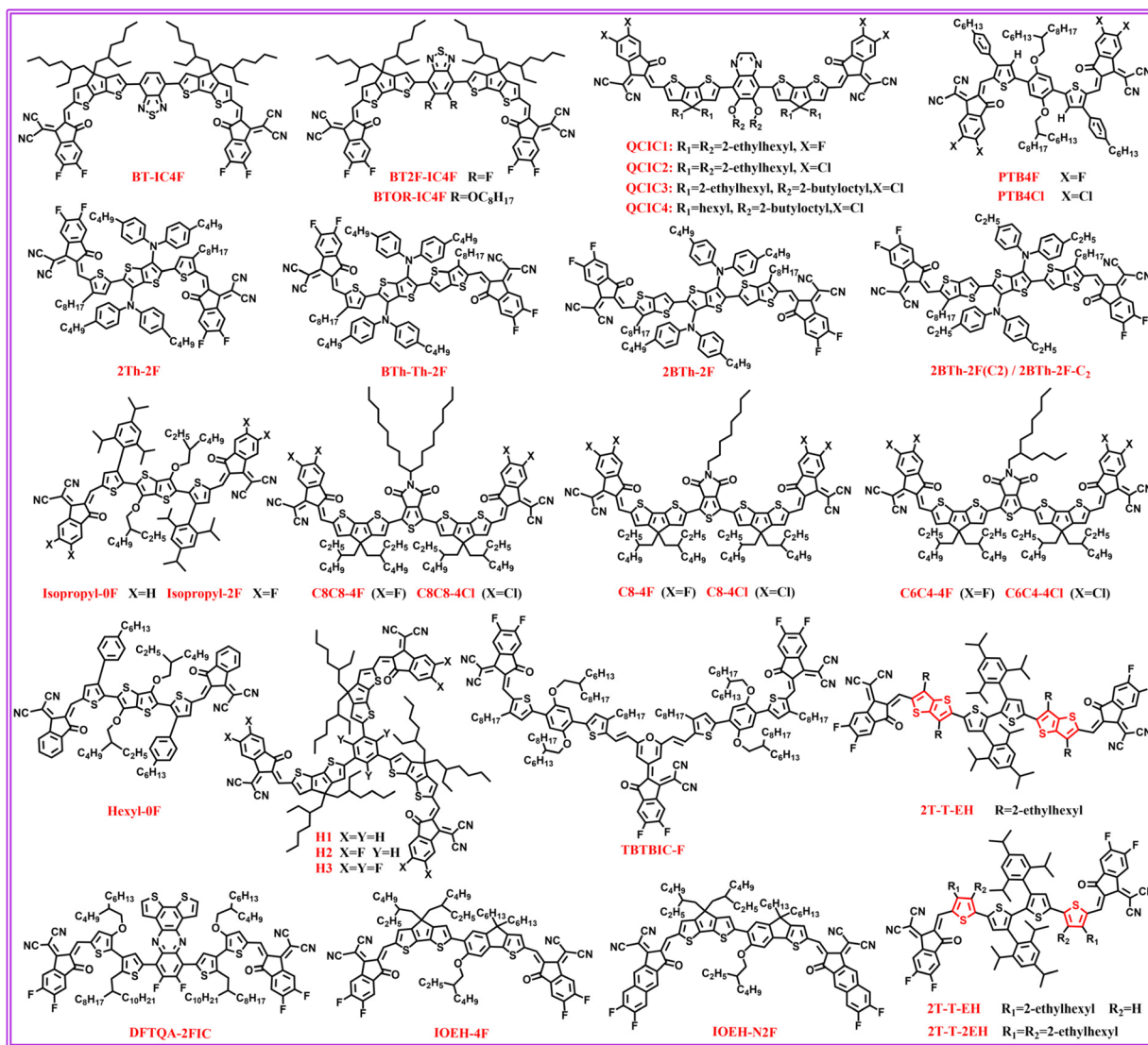
Fig. 17 Chemical structures of NFRAs regulated by C8 combinatorial strategies.
