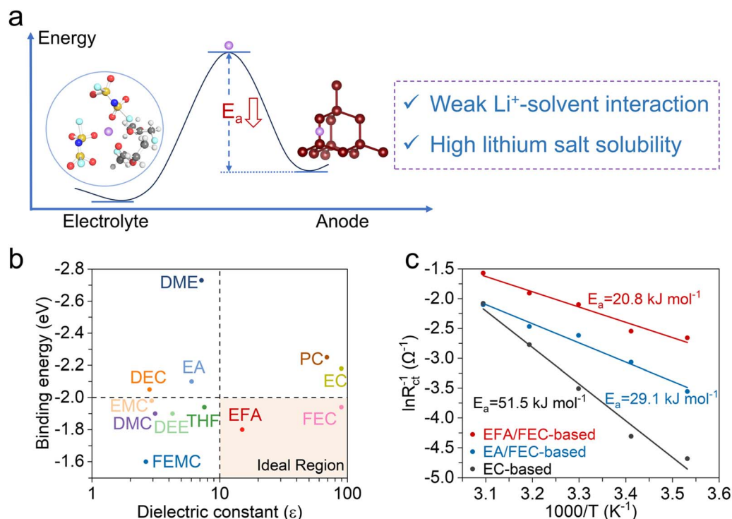
Fig. 1 Design principle of the electrolyte. (a) Schematic illustration of energetic coordinates for " \text{Li}^+ desolvation" at the silicon/electrolyte interface. (b) Diagram of binding energy and dielectric constant for solvents. 37,39 (c) Arrhenius curves and the corresponding activation energies ( E_a ) of the different electrolytes. EFA/FEC-based: 1.5 M LiFSI and 0.1 M LiDFOB in EFA/FEC (8 : 2, by volume). EA/FEC-based: 1.5 M LiFSI and 0.1 M LiDFOB in EA/FEC (8 : 2, by volume). EC-based: 1 M \text{LiPF}_6 in EC/DMC (1 : 1, by volume) with 10 wt% FEC.
