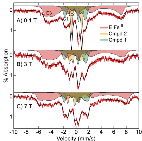
Fig. 5 Mössbauer spectra (A–C) red vertical bars) of oxidized Ne bCcP at pH 8.6 reacted with 15 equivalents H 2 O 2 recorded at 4 K in the magnetic fields listed. The black traces and filled areas are simulations (see text) for the parameters of Table 1.
