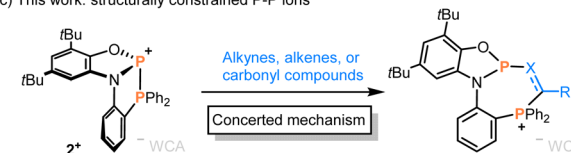
Scheme 1 (a) Phosphinophosphination of electron deficient (with A ) or electron-rich terminal alkynes and diazo compounds (with B ). (b) Structurally constrained phosphenium ions applied for E–H, C–H, and H–H bond activation (E = N, O, Si, B). (c) This work: phosphinophosphination of unsaturated compounds by a concerted mechanism.
