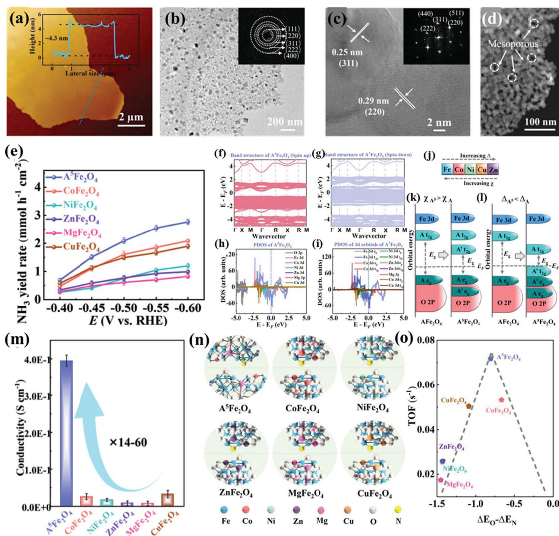
Fig. 11 HESs for the electrochemical \text{NO}_3^- RR. (a) Thickness measurement of ( \text{Co}_{0.2}\text{Ni}_{0.2}\text{Zn}_{0.2}\text{Mg}_{0.2}\text{Cu}_{0.2} )Fe 2 O 4 (A 5 Fe 2 O 4 ) nanosheets by AFM, (b) TEM (the inset shows the SAED patterns), (c) HRTEM, and (d) HAADF-STEM image of A 5 Fe 2 O 4 , (e) NH 3 yield rate of A 5 Fe 2 O 4 and binary spinel oxides at different potentials, the calculated band structure of A 5 Fe 2 O 4 (f) (spin up) and (g) (spin down), (h and i) PDOS for A 5 Fe 2 O 4 , (j) trends in crystal field splitting \Delta and electronegativity \chi for the five metals of the HES, schematic illustration that (k) adding a transition metal with greater electronegativity reduced the bandgap energy by introducing states between the e_g and t_{2g} states of the original transition metal and (l) adding a transition metal of lower crystal field splitting reduced the bandgap energy both by introducing new occupied t_{2g} states above the e_g states of the original transition metal and by lowering its unoccupied t_{2g} states, (m) electron conductivity of all spinel oxides, (n) optimized structural model of adsorbate nitrogenous compounds (*NO, *N, *NH, *NH 2 , and *NH 3 ) and oxycompounds (*NO 3 , *NO 2 , and *OH) on A 5 Fe 2 O 4 and other binary spinels, and (o) a volcano-type relationship between the binding difference of O and N ( \Delta E_{\text{O}} - \Delta E_{\text{N}} ) and TOF values of different spinel catalysts. Reproduced with permission. 22 Copyright 2022, John Wiley and Sons.
