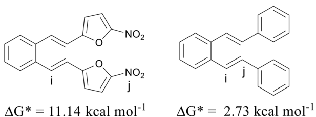
Fig. 10 Positions of site “i” required for the reaction to proceed and the most favorable protonation site “j” for compounds 13 and 14, together with the differences in Gibbs free energy between protonated species “i” and “j”, \Delta G^* .
