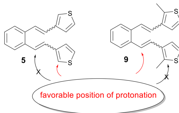
Fig. 2 Favorable protonation position.
