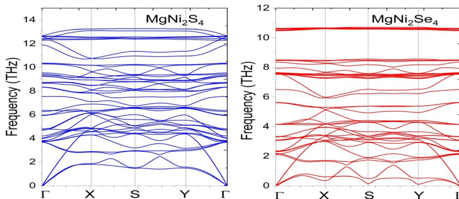
Fig. 3 Phonons dispersion plots of \text{MgNi}_2\text{X}_4 ( \text{X} = \text{S}/\text{Se} ).
