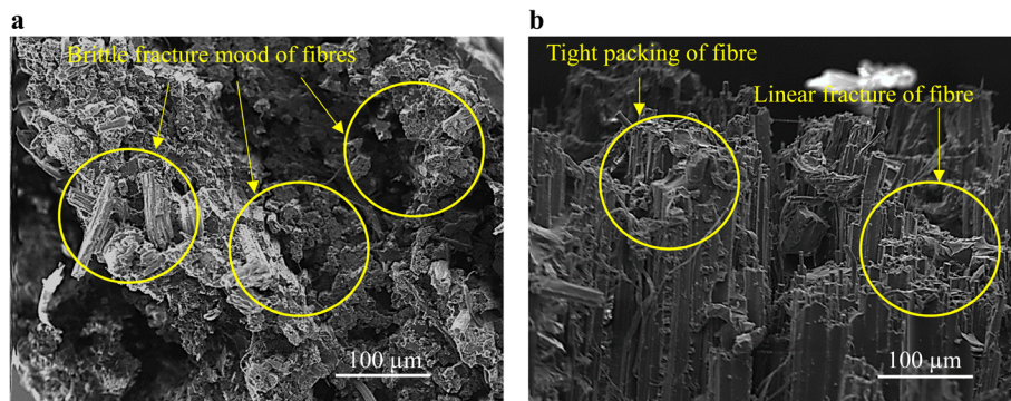
Fig. 9 (a) SEM fracture specimen of filed retted jute roving composite without GO coating at 250× magnification, (b) SEM fracture specimen of field retted jute roving composites with GO coatings at 250× magnification.
