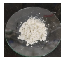
3a (1.35 g, 10 mmol) 4a (1.29 g, 96% isolated yield)
