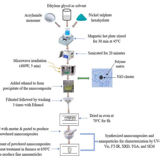
Fig. 1 Synthesis route of PAM/NiO NC by microwave technology.
