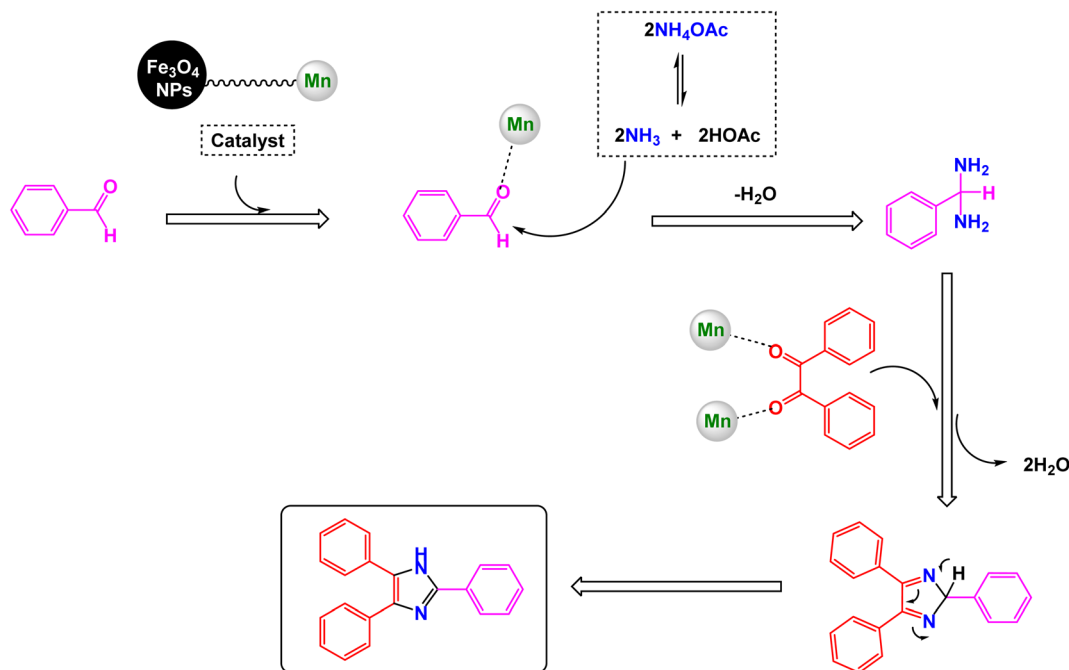
Scheme 19 Suggested mechanism for synthesis of triaryl imidazoles [catalysis by Fe 3 O 4 @SiO 2 -ABMA-MnCl 2 nanocomposite].
