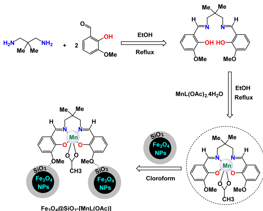
Scheme 7 General method to construct the \text{Fe}_3\text{O}_4@\text{SiO}_2\text{--}[\text{MnL}(\text{OAc})] nanocomposite.
