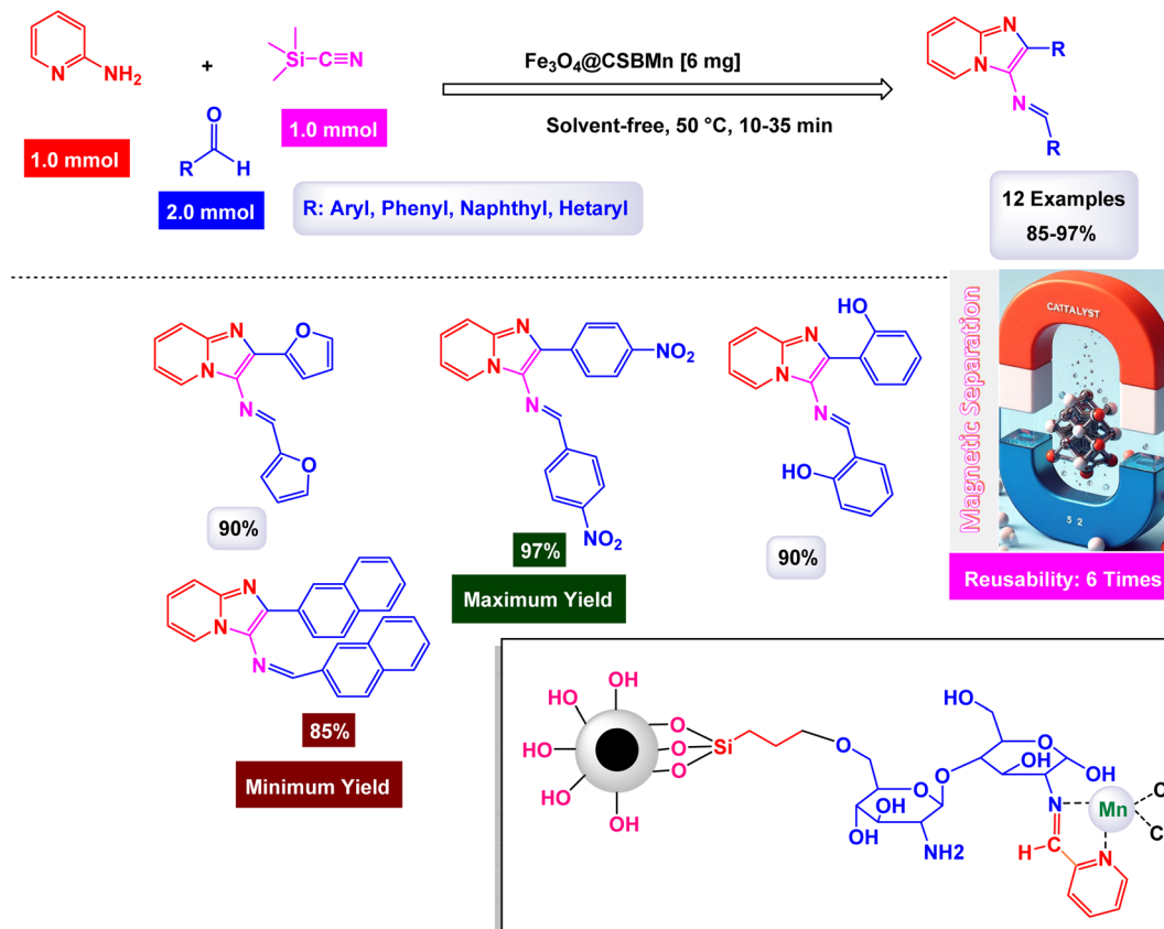
Scheme 31 Synthesis of imidazo[1,2-a]pyridines [catalysis by \text{Fe}_3\text{O}_4@\text{CSBMn} nanocomposite].
