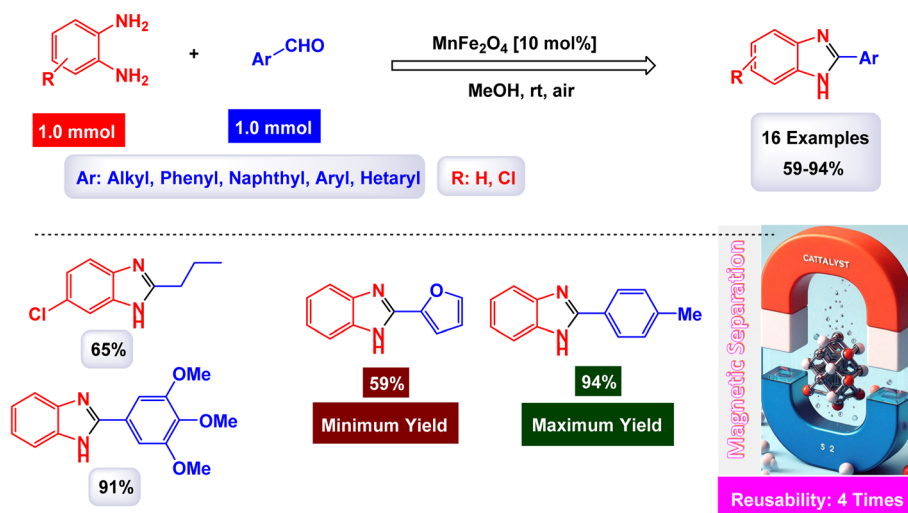
Scheme 20 Synthesis of benzimidazoles [catalysis by MnFe 2 O 4 nanocomposite].
