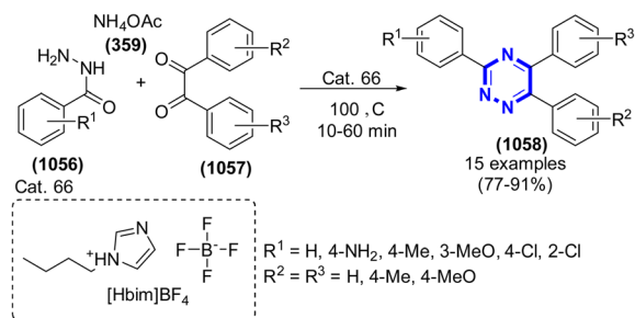
Scheme 294 Synthesis of 1,2,4-triazines catalyzed by Cat. 66.
