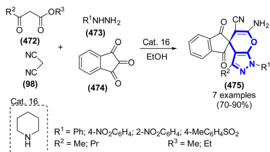
Scheme 127 Synthesis of spiro-pyranopyrazoles and oxa-aza-[3.3.3]propellanes catalyzed by \text{Cat. 16} in ethanol.
