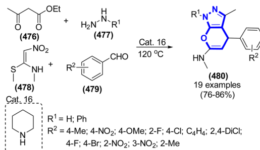
Scheme 128 Synthesis of pyranopyrazole frameworks catalyzed by \text{Cat. 16} .
