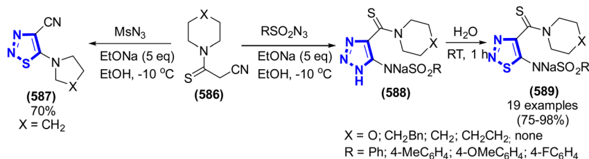
Scheme 158 Synthesis of 4,5-functionalized 1,2,3-thiaziazoles.
