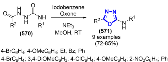
Scheme 152 Synthesis of oxadiazole moieties catalyzed by NEt 3 .
