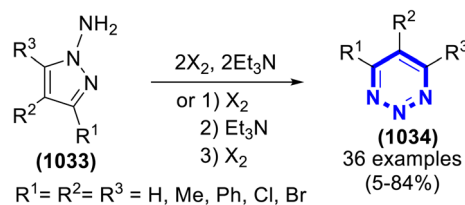
Scheme 288 Synthesis of halogenated and unhalogenated 1,2,3-triazines.
