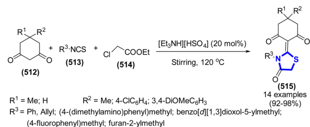
Scheme 136 Synthesis of thiazolidine/oxazolidine derivatives catalyzed by [\text{Et}_3\text{NH}][\text{HSO}_4] .
