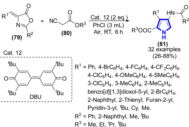
Scheme 21 Preparation of 2,3,4-trisubstituted pyrroles catalyzed by Cat. 12.
