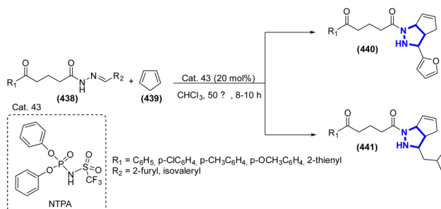
Scheme 118 Creation of novel pyrazolidines through [3 + 2] cycloaddition.
