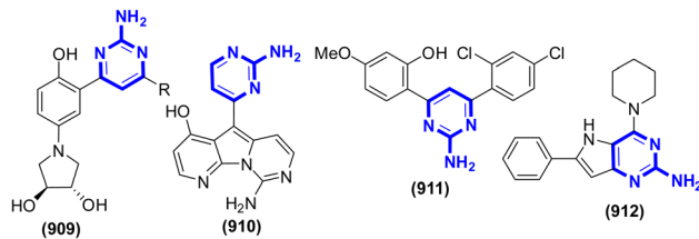
Scheme 258 Chemical structures of bioactive compounds containing a benzo[4,5]imidazo[1,2-a]pyrimidine framework.
