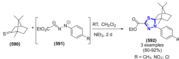
Scheme 159 Synthesis of 1,3,4-thiaziazole frameworks.
