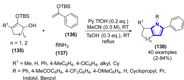
Scheme 38 Synthesis of tetrahydrocyclopenta[ b ]pyrroles catalyzed by Py TFOH.
