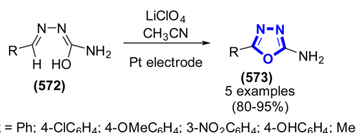
Scheme 153 Synthesis of oxadiazole frameworks catalyzed by LiClO 4 via an electrolysis method.
