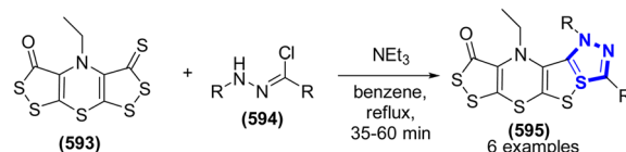
Scheme 160 Synthesis of dithiolo[1,4]thiazines catalyzed by NEt 3 .
