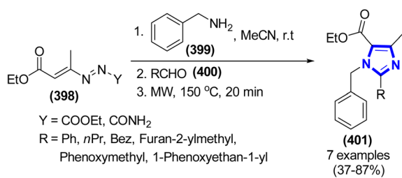
Scheme 106 Synthesis of 2-substituted 3 H -imidazole-4-carboxylates under MW.
