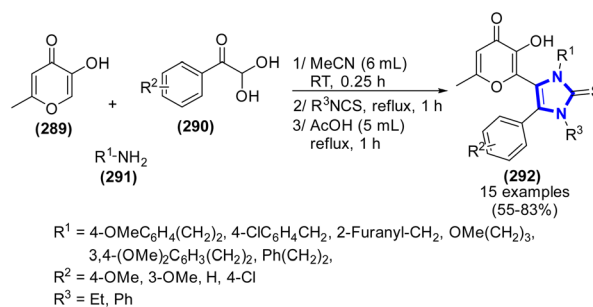
Scheme 78 Synthesis of imidazole-2-thione derivatives.
