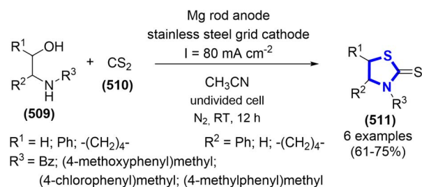
Scheme 135 Synthesis of thiazoline-2-thione derivatives in the presence of \text{CS}_2 .
