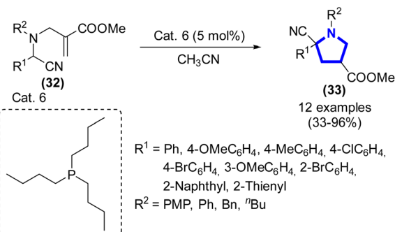
Scheme 9 Synthesis of 2,4-disubstituted pyrrolidines catalyzed by Cat. 6.
