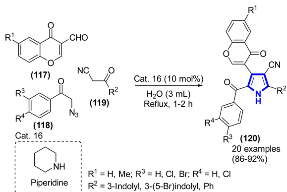
Scheme 33 Synthesis of chromenopyrrole catalyzed by Cat. 16.
