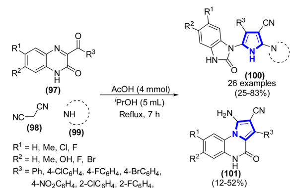
Scheme 27 Synthesis of pyrroles catalyzed by acetic acid.
