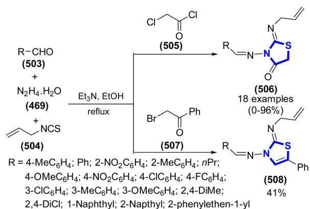
Scheme 134 Synthesis of a wide range of thiazolidine-4-one and 3 H -thiazoles catalyzed by \text{Et}_3\text{N} .
