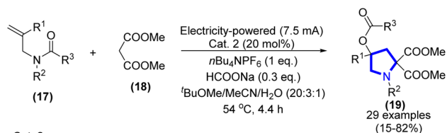
Scheme 4 Synthesis of pyrrolidine and tetrahydropyridine derivatives catalyzed by Cat. 2.
