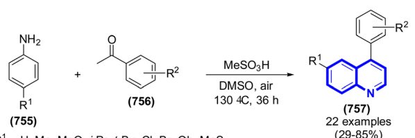
Scheme 213 Synthesis of quinolines catalyzed by methanesulfonic acid.
