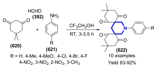
Scheme 169 Synthesis of piperidines catalyzed by 2,2,2-trifluoroethanol.
