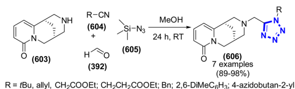
Scheme 163 Synthesis of tetrazole derivatives of cytosine.
