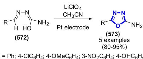
Scheme 153 Synthesis of oxadiazole frameworks catalyzed by LiClO 4 via an electrolysis method.
