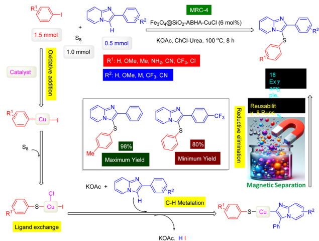
Scheme 4 \text{Fe}_3\text{O}_4@SiO_2\text{-ABHA-CuCl} nanomaterial ( MRC-4 ) catalyzed synthesis of diaryl sulfides infused with intricate imidazo[1,2- a ]pyridine scaffolds from S_8 .
