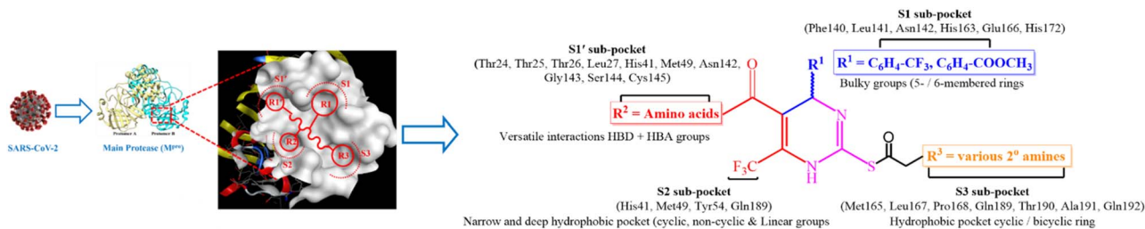
Fig. 4 Design strategy for SARS-CoV-2 M Pro inhibitors.
