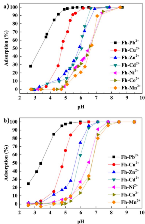
Fig. 2 Effects of pH on the sorption of 7 HMs on Fh in single (a) and competitive (b) system (mass-to-volume ( m/v ) = 5.0 \text{ g L}^{-1} , I = 0.01 \text{ mol L}^{-1} NaCl, T = 25 \text{ }^\circ\text{C} , C_M = 1.0 \times 10^{-3} \text{ mol L}^{-1} ).
