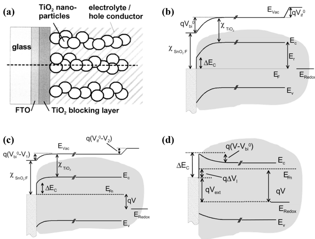
Fig. 18 (a) Schematic side view of a DSSC comprising nanocrystalline 1-D \text{TiO}_2 photoanodes and electrolyte, (b and c) schematic band model of DSSC under dark and light conditions, where the interfacial band bending arises due to the negative charges present in the electrolyte, and (d) detailed band diagram where light-induced V exceeds the V_{\text{bi}} .
