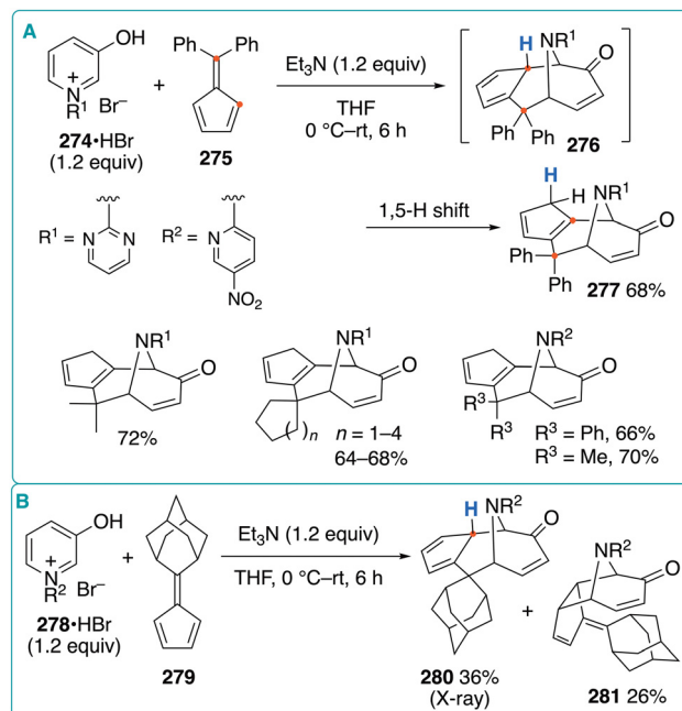
Fig. 38 (A) (5 + 6) cycloaddition of N-heterocycle-substituted oxidopyridinium betaines with fulvenes. (B) Reaction of N -(5-nitropyridin-2-yl)-substituted oxidopyridinium with adamantane-derived fulvene.
