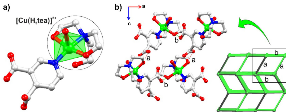
Fig. 2 Crystal structure fragments of compound 1 , [Cu(pdc)(H 3 tea)(H 2 O)]. (a) Polyhedral representation of the mononuclear copper(II) unit, [Cu(H 3 tea)] 2+ . (b) Left: H-bonded motifs a and b ; right: simplified representation of crystal packing with the sqc topology through H-bonding interactions. Solvent molecules and hydrogen atoms have been omitted for clarity. Color codes: Cu: green; O: red; N: blue; C: gray.
