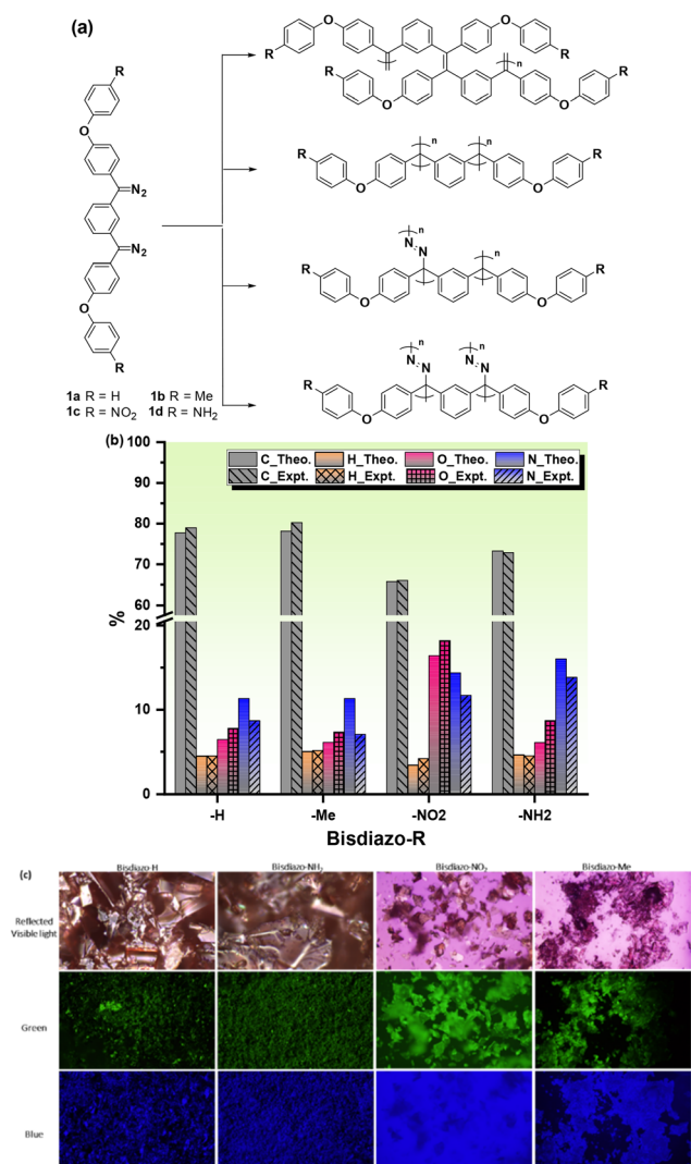
Fig. 1 (a) Chemical structures of bisdiazom-R compounds 1a–d and the possible repeating units of polymers under catalyst-free polymerization. (b) Elemental analysis and (c) optical and fluorescence images of bisdiazom-R compounds 1a–d with various terminal groups ( R = H , Me , NO_2 and NH_2 ).
