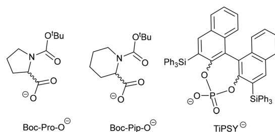
Fig. 4 Chiral anionic ligands for zinc(II). Boc-Pro-O − , Boc-Pip-O − and TIPSYP − are derived from N -(tert-butoxycarbonyl)-proline, N -(tert-butoxycarbonyl)-piperidine and 3,3'-bis(triphenylsilyl)-1,1'-binaphthyl-2,2'-diyl hydrogenphosphate respectively.
