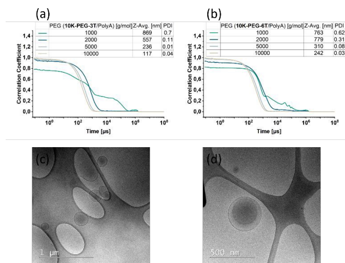
Fig. 3: DLS measurements to investigate the influence of PEG chain length on the nanoparticle formation of PEG-3T /PolyA (a), and PEG-6T /PolyA (b). The concentrations of PEG-3T and PEG-6T were 80 μM and the polyA concentration was 720 μM. The solvent used was 1X PBS. The table shows the mean value of the Z-average and the PDI of three individual measurements. Cryo-TEM images of 5K-PEG-3T /PolyA. The sizes of the scale bars are 1 μm (c) and 500 nm (d).
