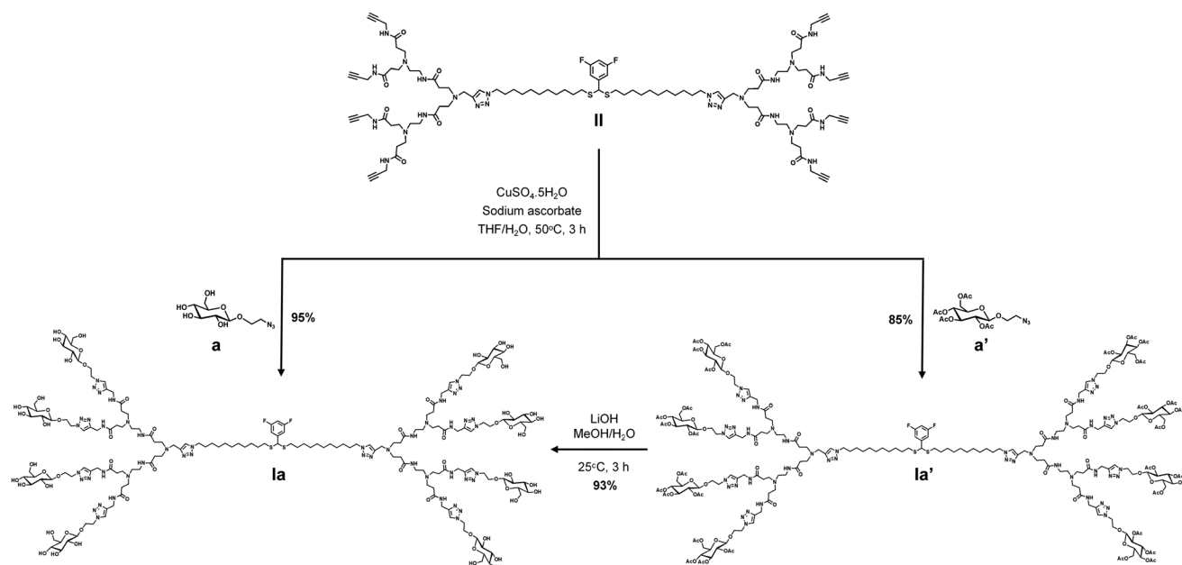
Fig. 3 Synthesis of the bola-amphiphilic glucose-dendrimer ( 1a ) using an unprotected carbohydrate derivative (left) and a protected carbohydrate unit (right).
