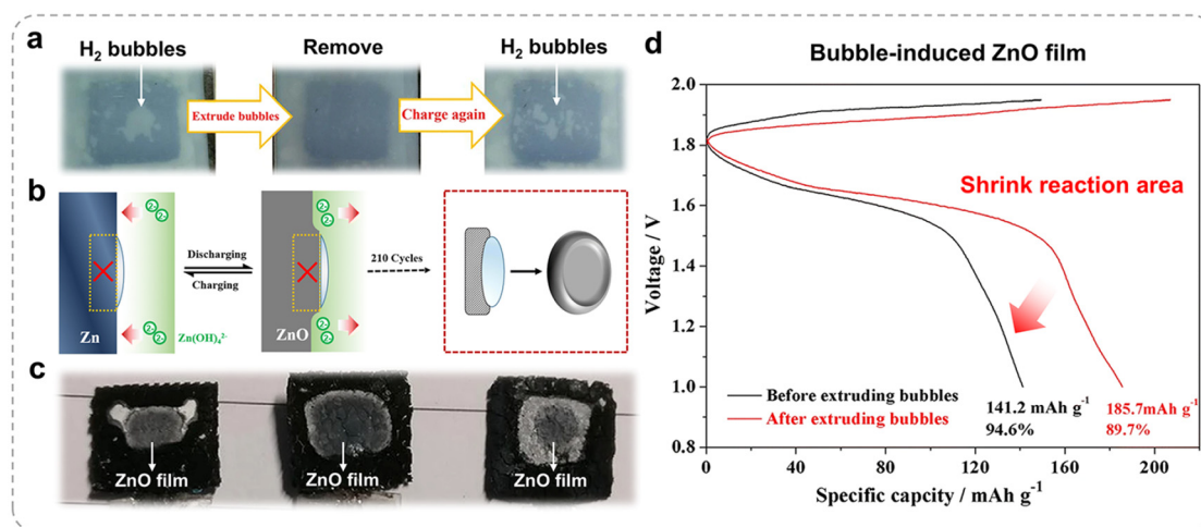
Fig. 5 (a) Hydrogen bubble formation on the back of a Zn electrode. (b) Schematic diagram of the hydrogen bubble effect on Zn electrode deformation. (c) Zn anode after 210 cycles. (d) Electrochemical performance before/after bubble extrusion. Reproduced from ref. 37 with permission from Springer, copyright 2021.
